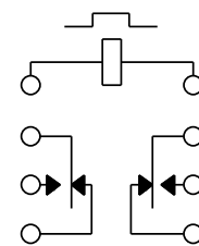
TERMINAL VIEW
