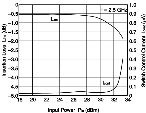
RFC-RF1/RF2 INSERTION LOSS, I_{\text{cont}} vs. INPUT POWER
