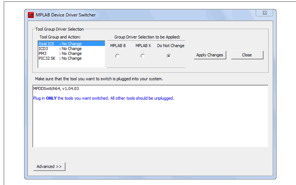
FIGURE 2-1: SWITCHER UTILITY
