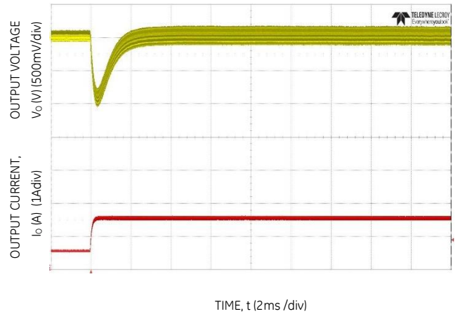
Figure 10. Transient Response to Dynamic Load Change from 0.6 to 1.6A at 12Vin, C_{out}=10 \times 4.7\mu\text{F} , C_{Tune}=560\text{pF} , R_{Tune}=40.2\text{k}
