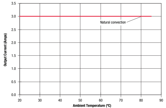
OKL-T/3-W12 Maximum Current Temperature Derating at Sea Level (Vin = 12V, Vout = 0.591V)
