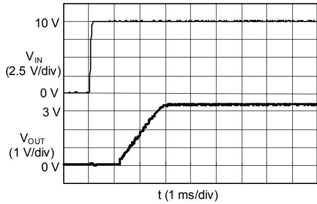
(4) S-8540C33FN ( V_{IN} : 0 \rightarrow 10 V)
