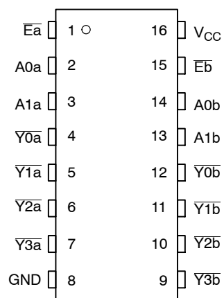
Figure 1. Pin Assignment
