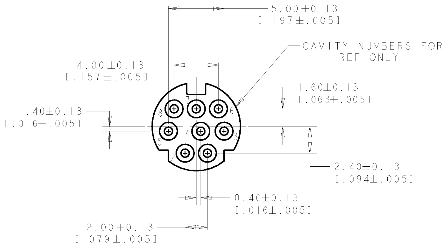
DETAIL D 8 PIN FACE
