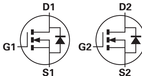
Equivalent Circuit
