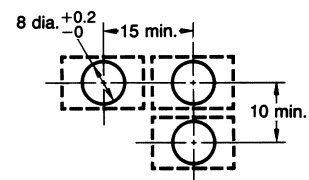
Panel cutout
