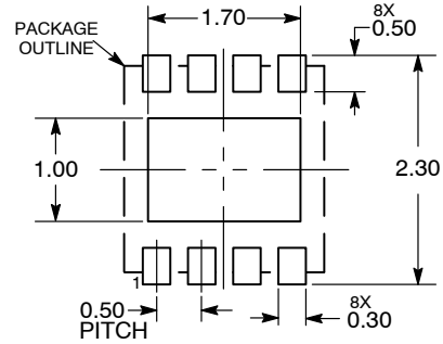
DIMENSIONS: MILLIMETERS
