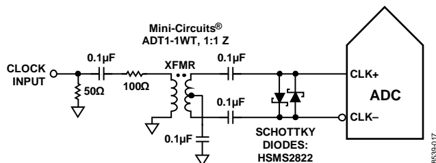
Figure 47. Transformer-Coupled Differential Clock (3 MHz to 200 MHz)
