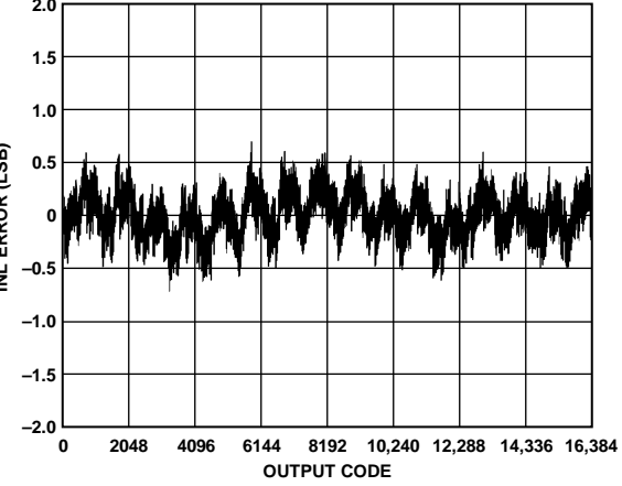
Figure 15. AD9649-80 INL with f_{IN} = 9.7 MHz
