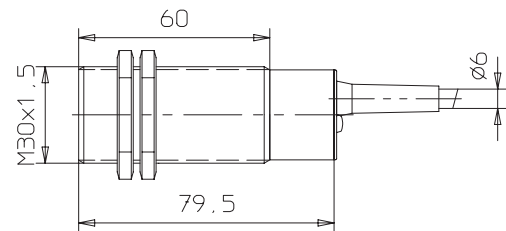
E2EL-X15M□-L 2M
