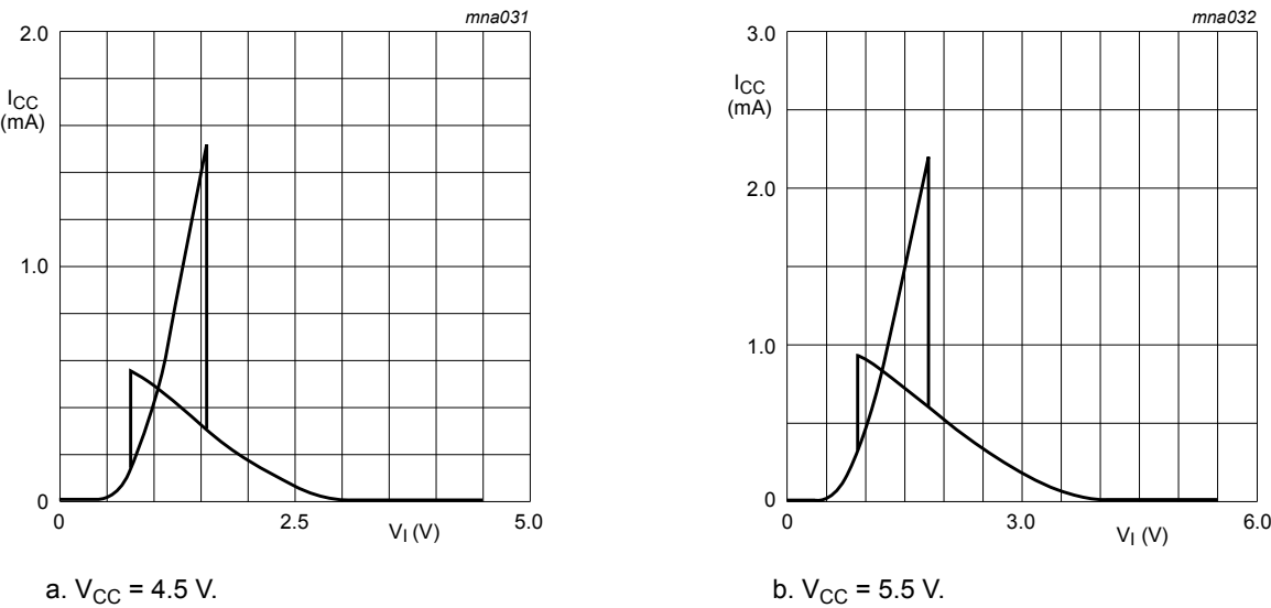
Fig. 8. Typical 74HCT3G14-Q100 transfer characteristics
