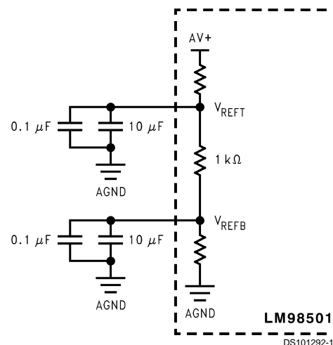
FIGURE 17. Reference Bypassing
