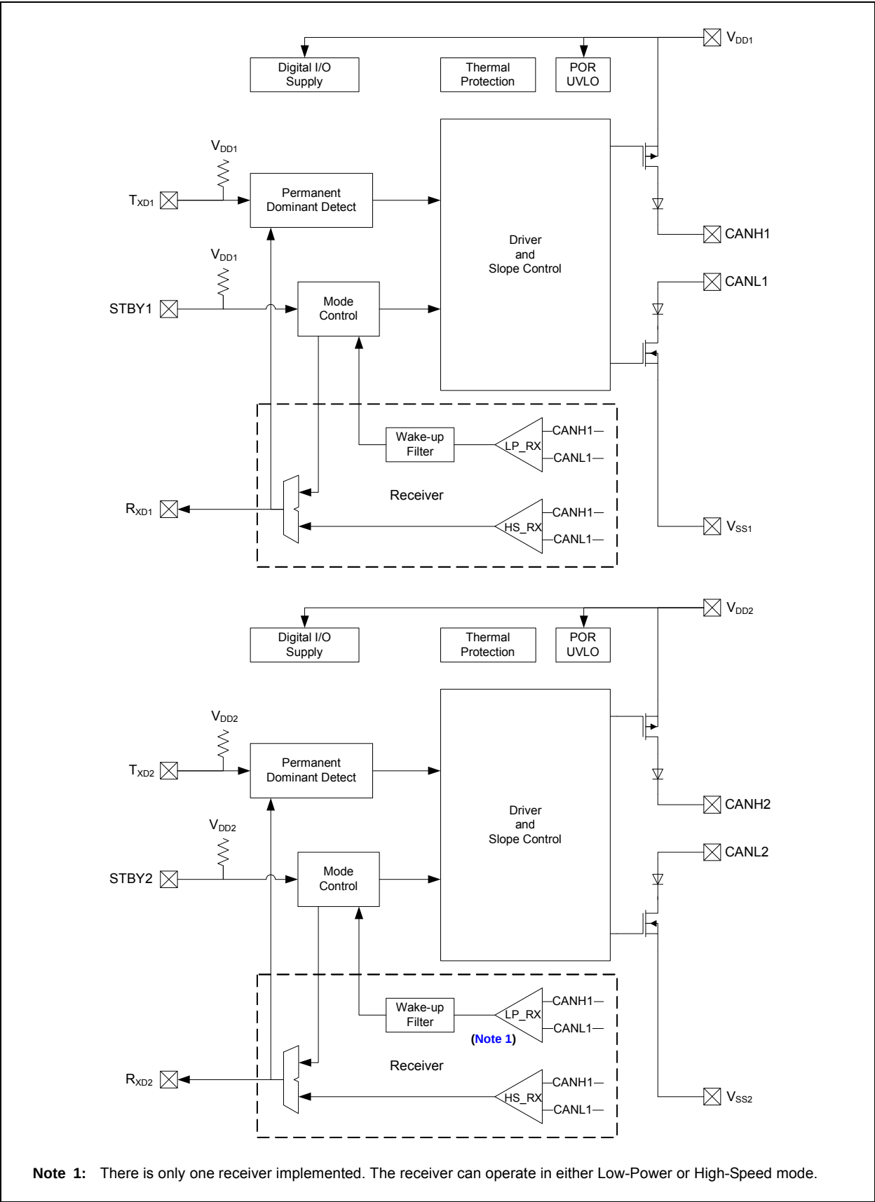
Device Block Diagram
