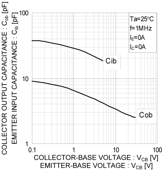
Fig.10 Emitter Input Capacitance vs. Emitter-Base Voltage Collector Output Capacitance vs. Collector-Base Voltage
