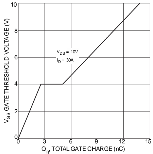
Figure 12 Gate Charge
