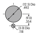
Maximum Panel Thickness: .185" (4.7mm)
