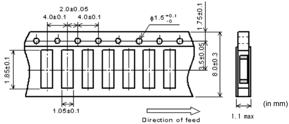
Dimension of the Cavity is measured at the bottom side.
