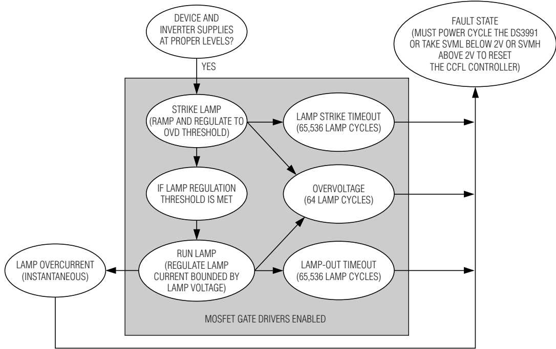
Figure 3. Fault-Handling Flowchart
