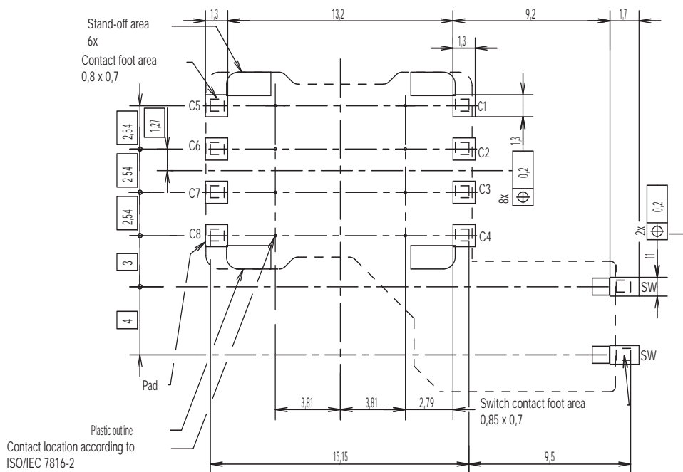
RECOMMENDED PCB BOARD LAYOUT (Component side)
