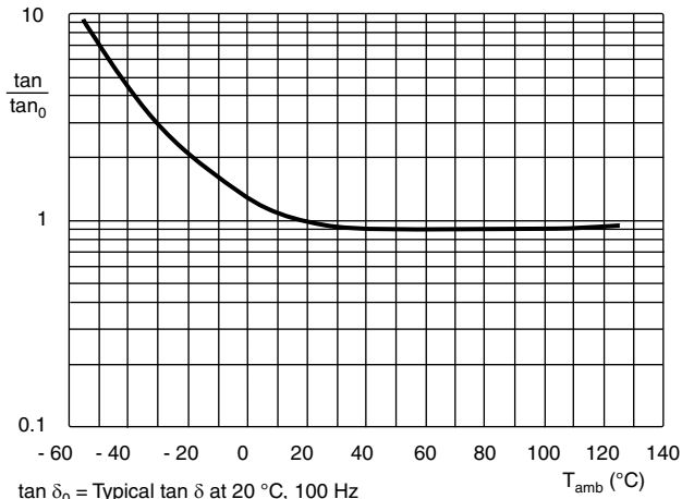
Fig. 6 - Typical multiplier of dissipation factor (tan δ) as a function of ambient temperature
