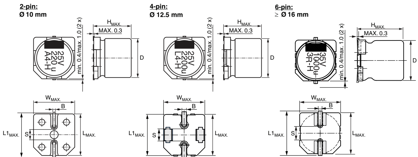
Fig. 2 - Dimensional outline
