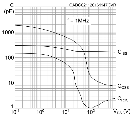
Figure 8: Capacitance variations
