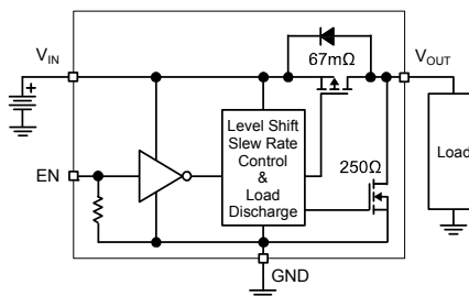
MIC94081 (ultra fast turn on with auto-discharge) MIC94083 (800μs soft-start with auto-discharge) MIC94085 (120μs soft-start with auto-discharge)
