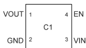
4-Pin (0.85mm x 0.85mm) Thin MLF ® (Top View)
