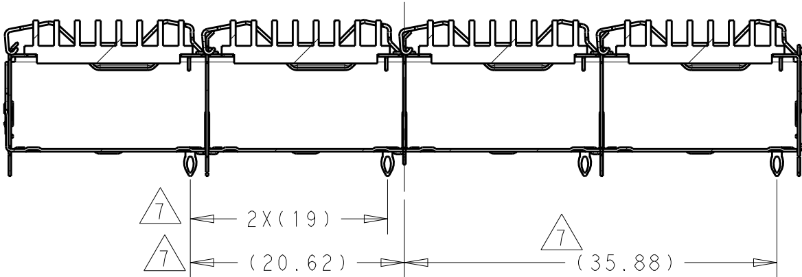
For 2343988-1/-2-3 WITH REAR EONS SECTION W-W
