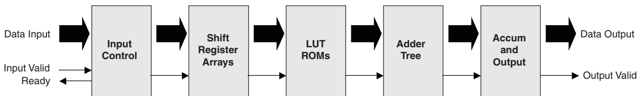
Figure 2-1. DA-FIR Filter Generator Block Diagram
