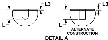
QFNW24 5x5, 0.65P CASE 484AF ISSUE A
