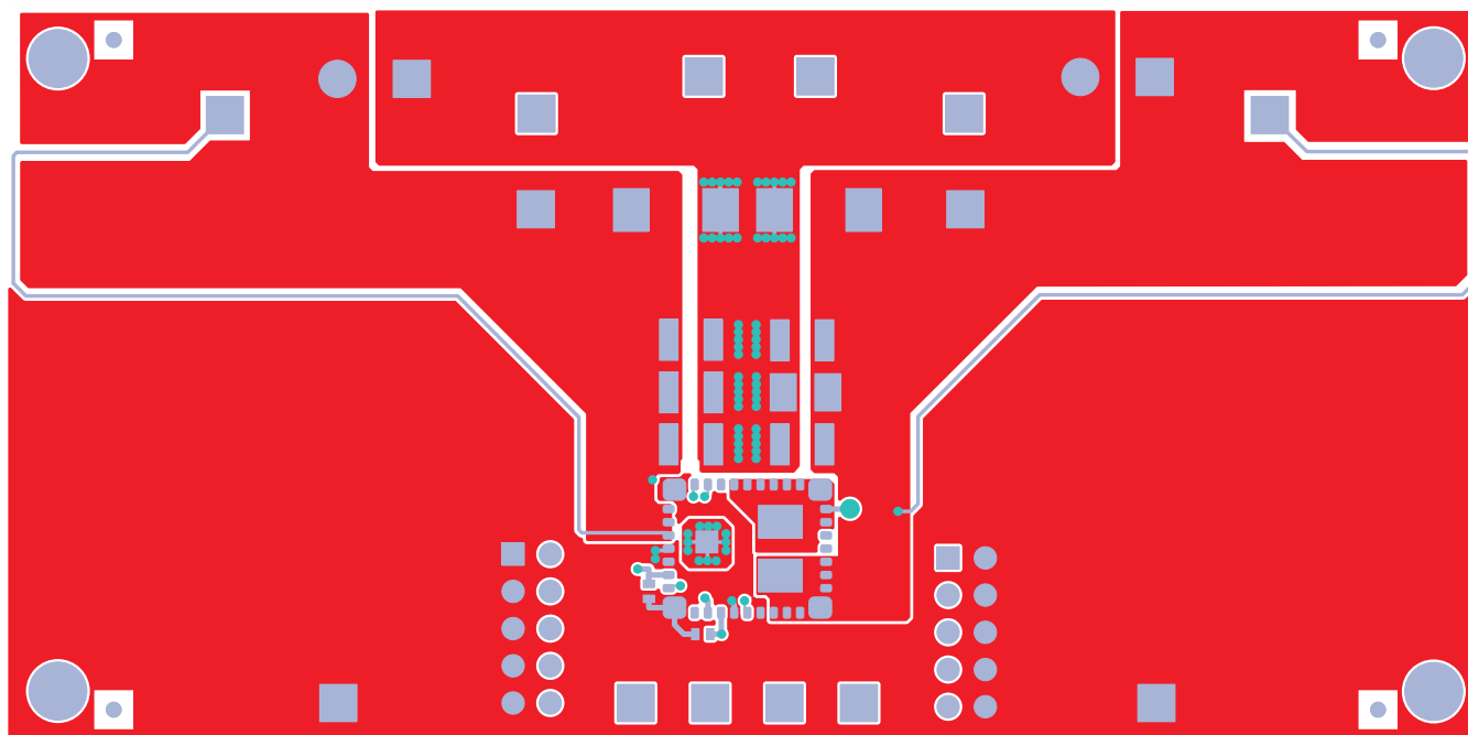
Figure 4. Top Layer
