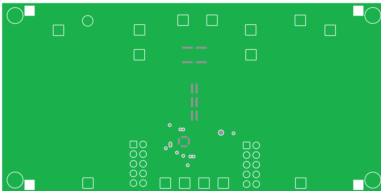
Figure 5. Internal 1 Layer
