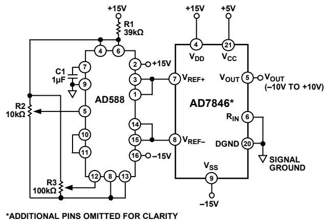
Figure 24. Bipolar \pm 10\text{ V} Operation
