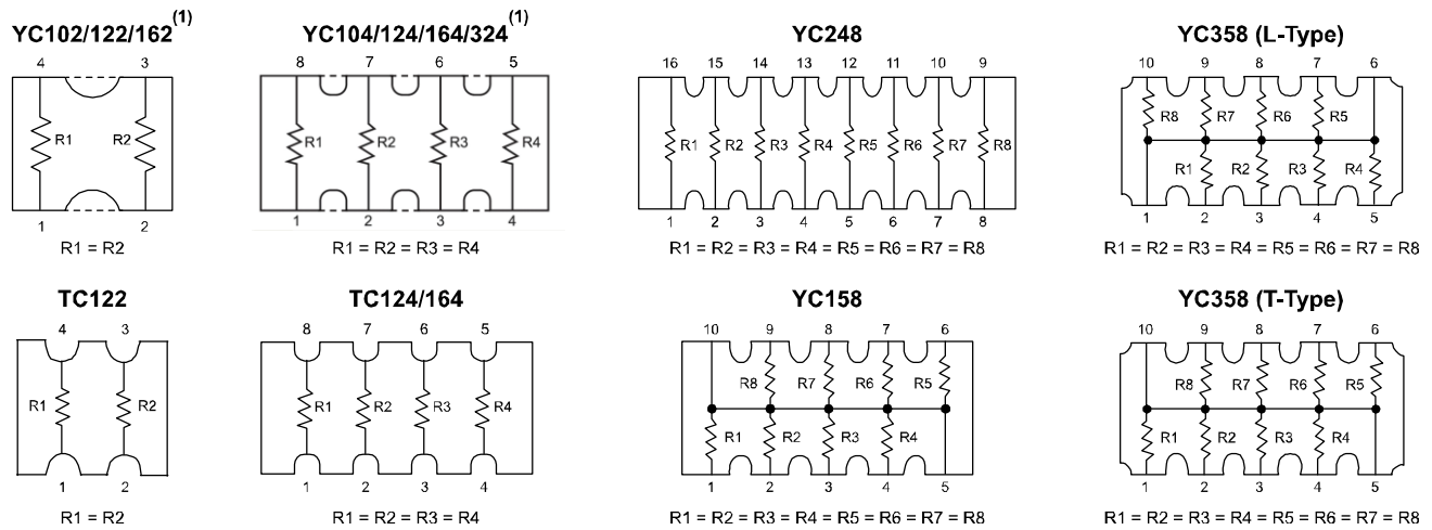
Fig. 11 Equivalent circuit diagram
