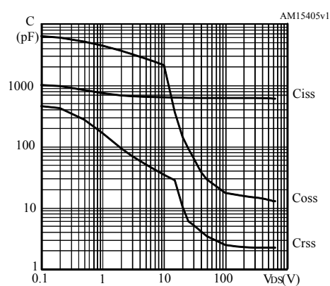
Figure 12. Capacitance variations
