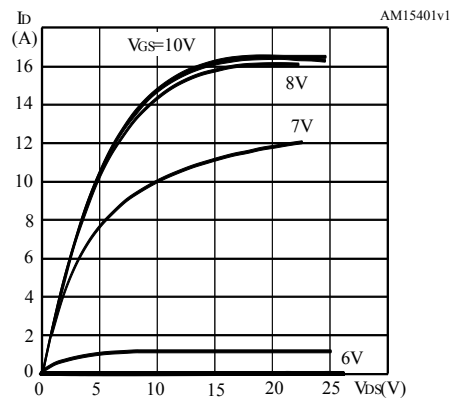
Figure 8. Output characteristics
