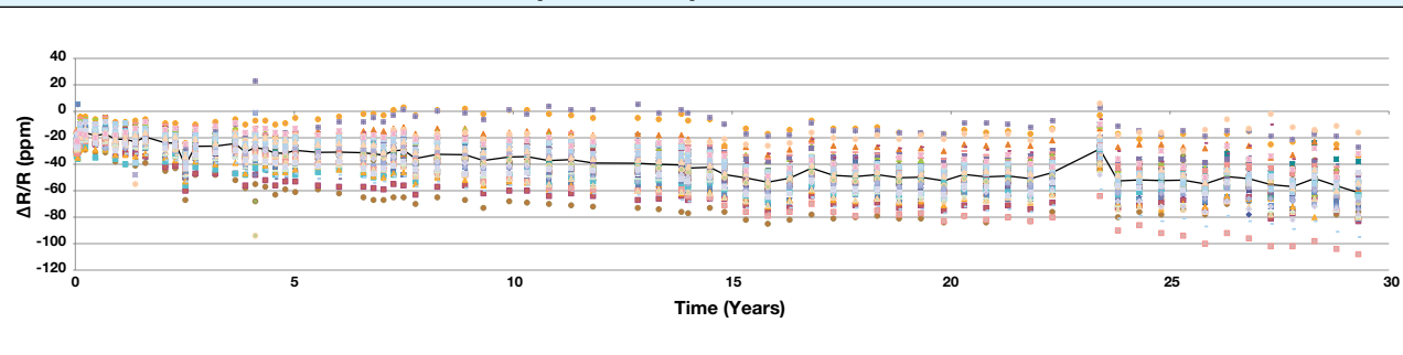
FIGURE 4 - THROUGH-HOLE STYLE (29 YEARS)
