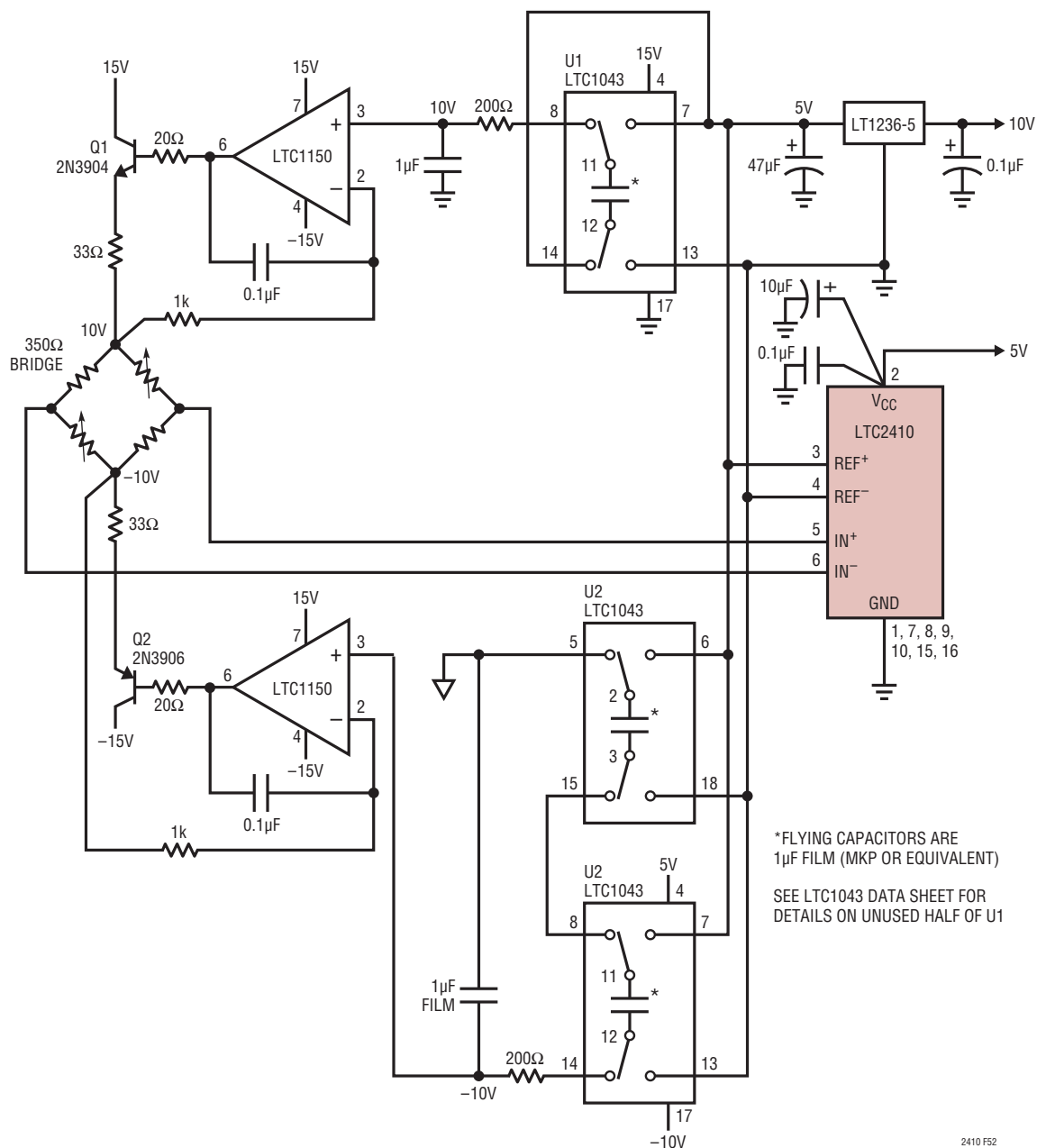
Figure 52. LTC1043 Provides Precise 4× Reference for Excitation Voltages
