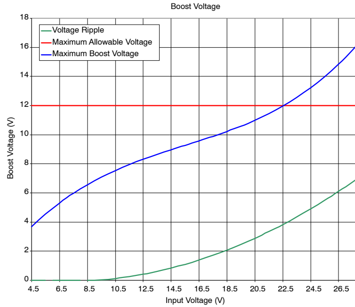
(Clarity on Boost Max and Ripple Def) Figure 32. Boost Voltage at 80% Duty Cycle
