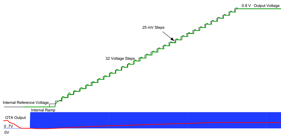
Figure 19. Soft-Start Details
