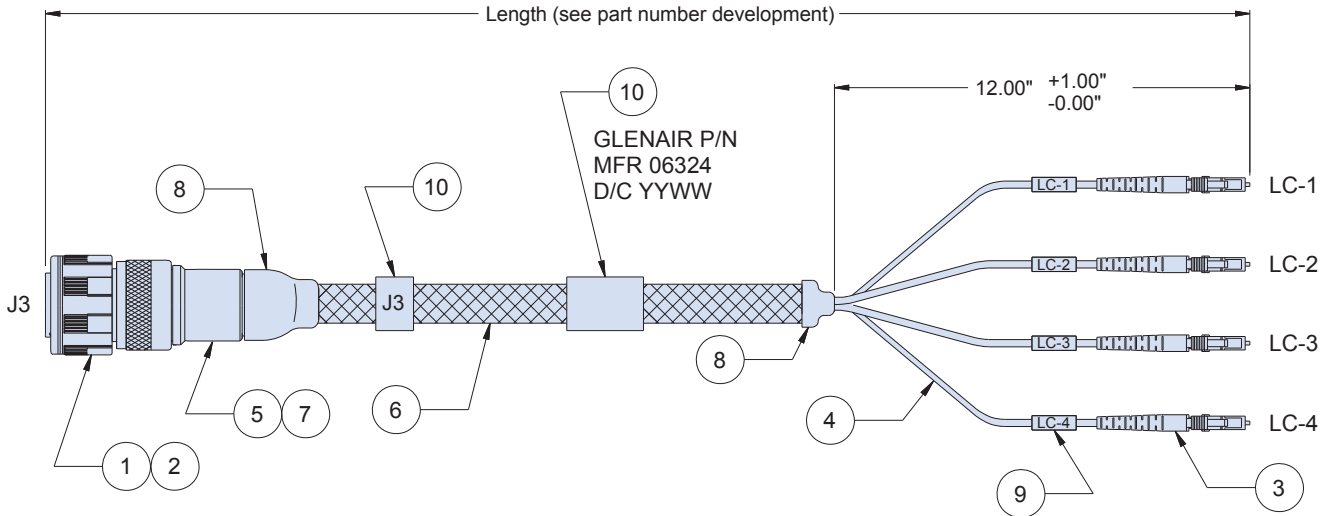
Connection Diagram
