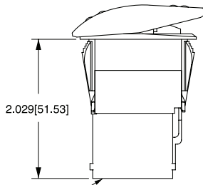
SWITCH SHOWN WITH VCH CONNECTOR 8 TERMINAL
