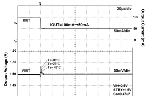
Fig 46. Load Response
