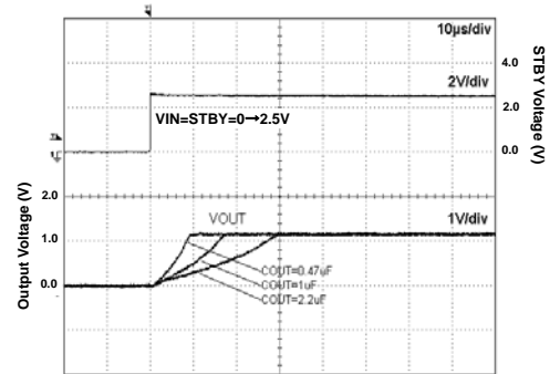
Fig 25. Start Up Time (VIN=STBY) Iout=200mA Iout=200mA
