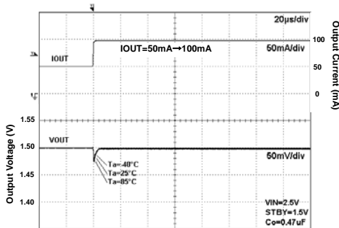
Fig 45. Load Response
