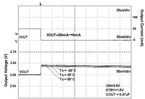
Fig 142. Load Response
