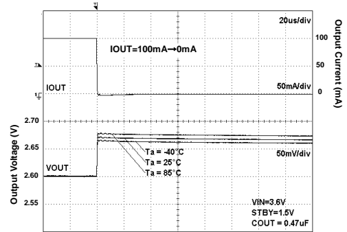
Fig 144. Load Response
