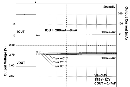
Fig 146. Load Response
