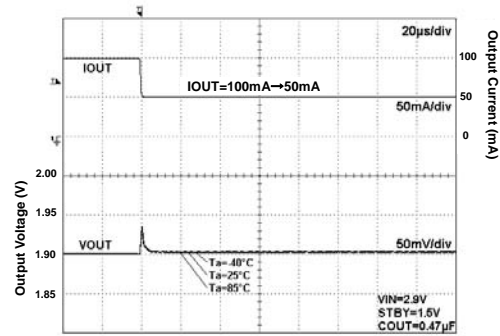
Fig 96. Load Response
