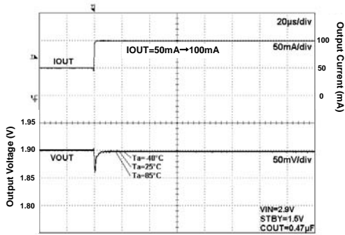
Fig 95. Load Response
