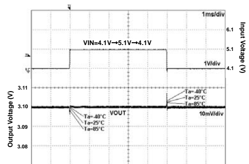
Fig 258. VIN Response
