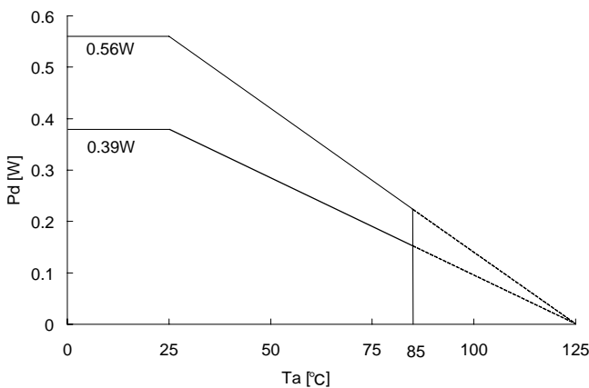
Fig. 285 SSON004X1010 Power dissipation heat reduction characteristics (Reference)
