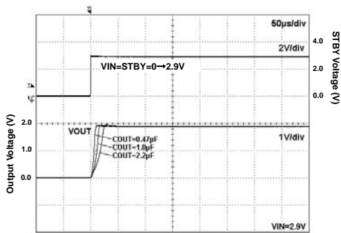
Fig 99. Start Up Time (VIN=STBY) Iout=0mA
