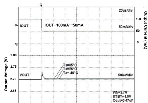
Fig 174. Load Response
