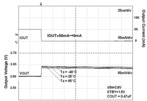
Fig 142. Load Response
