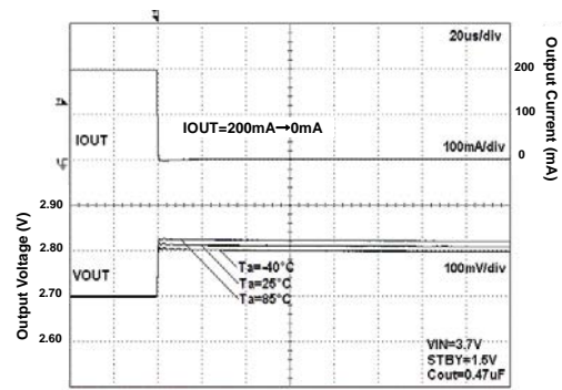
Fig 172. Load Response
