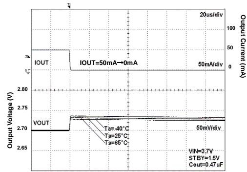
Fig 168. Load Response
