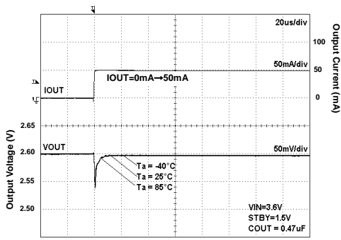
Fig 141. Load Response
