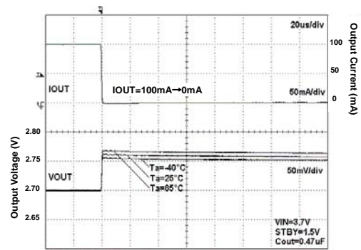
Fig 170. Load Response
