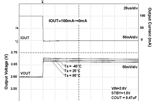
Fig 144. Load Response
