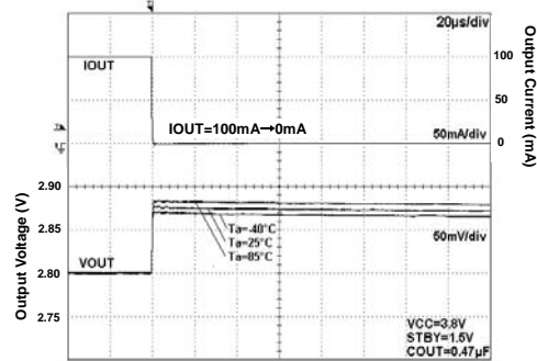
Fig 196. Load Response
