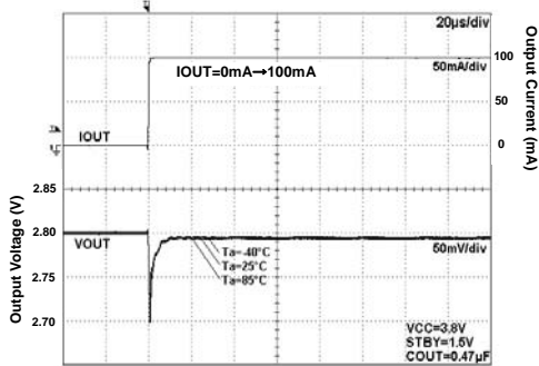
Fig 195. Load Response
