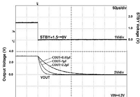
Fig 283. Discharge Time
