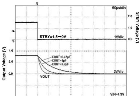
Fig 283. Discharge Time
