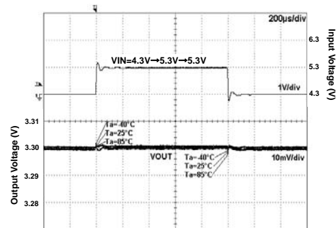
Fig 284. VIN Response
