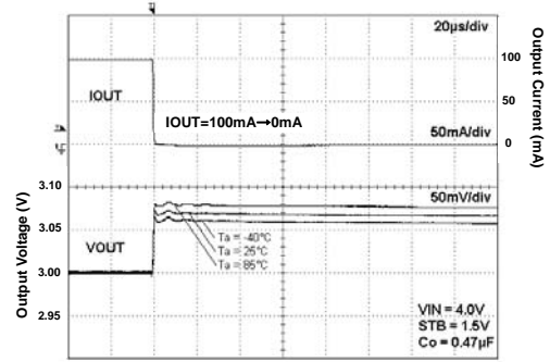
Fig 222. Load Response
