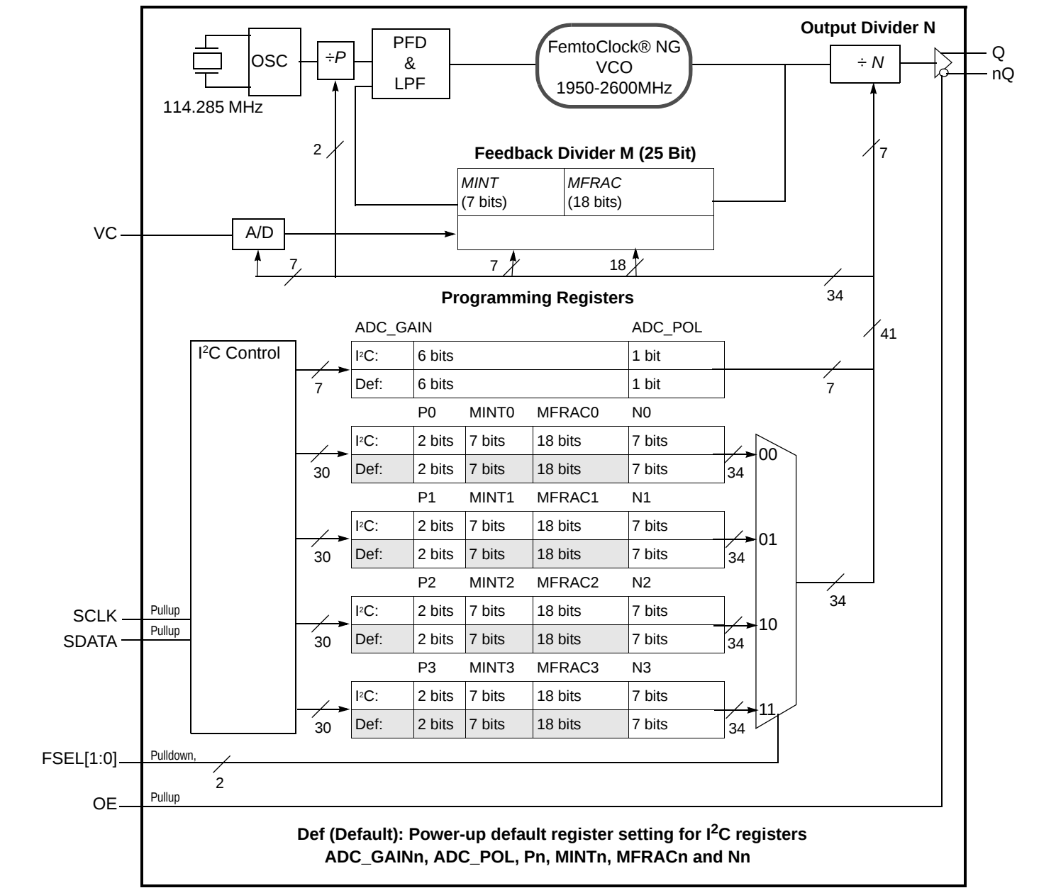
Block Diagram with Programming Registers
